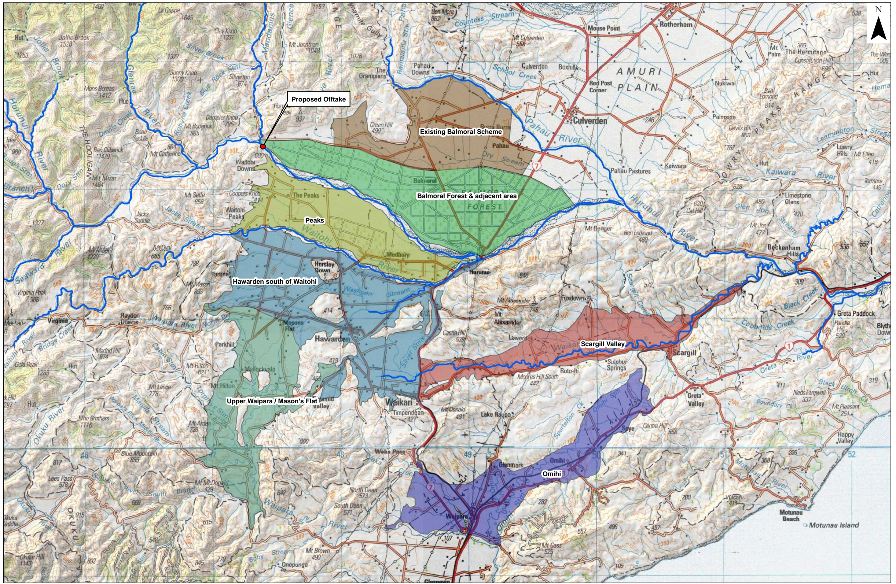
Figure A1 : Proposed Irrigation Area and Offtake
