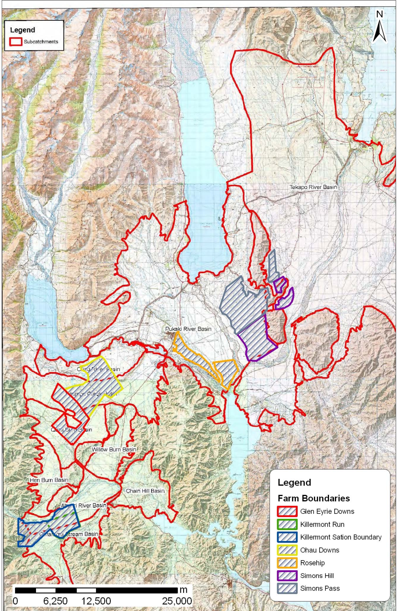
Figure 2: Groundwater subcatchment boundaries
