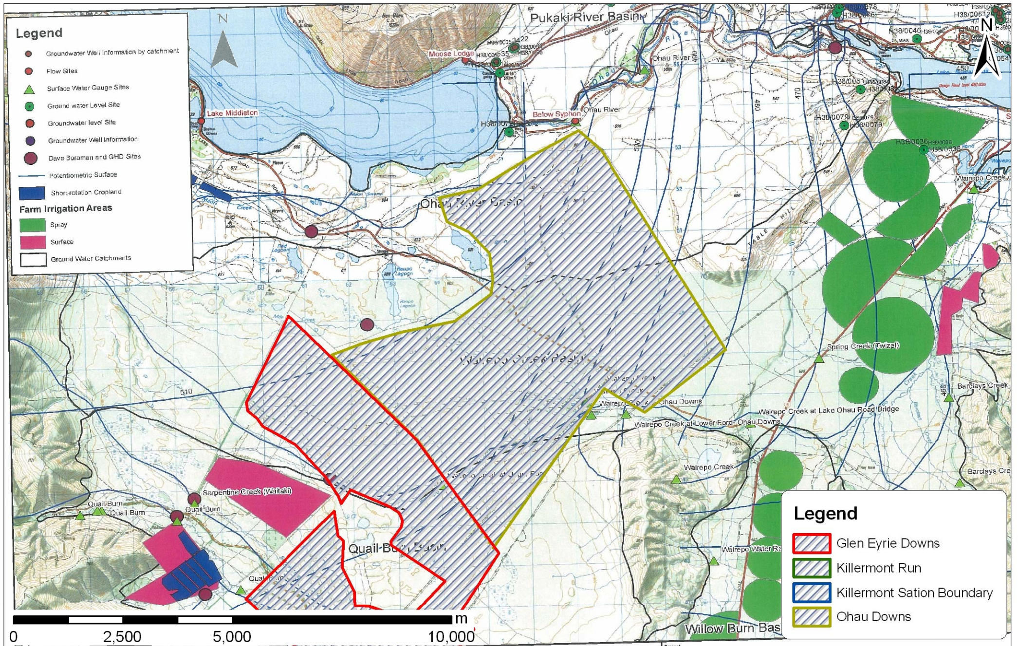
Figure 5: Wairepo Creek groundwater subcatchment
