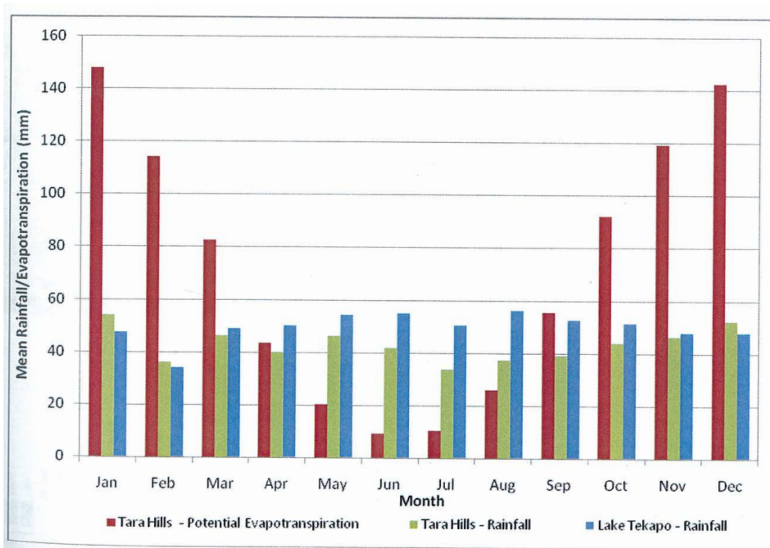
Figure 12: Comparison of potential evapotranspiration and rainfall at Tara Hills as well as rainfall at Lake Tekapo, the data covers the period 1950 to 2007 (data source: NIWA 2008). Image sourced from Cooksey, 2008
