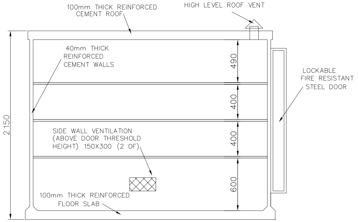
SIDE ELEVATION
